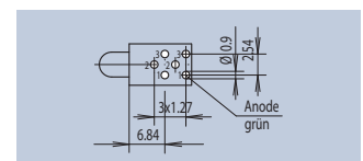
Bohrbild · Drilling Scheme
